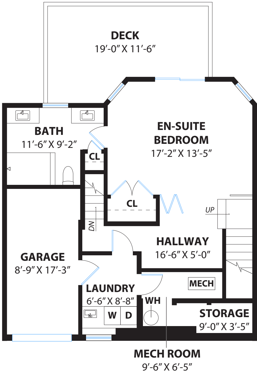
LOWER FLOOR 1
