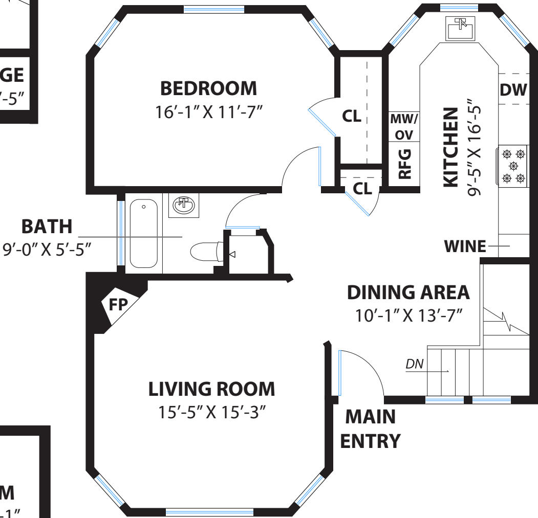
MAIN FLOOR
