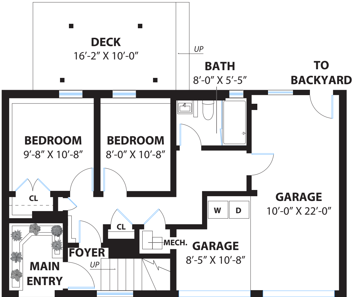
LOWER LEVEL
