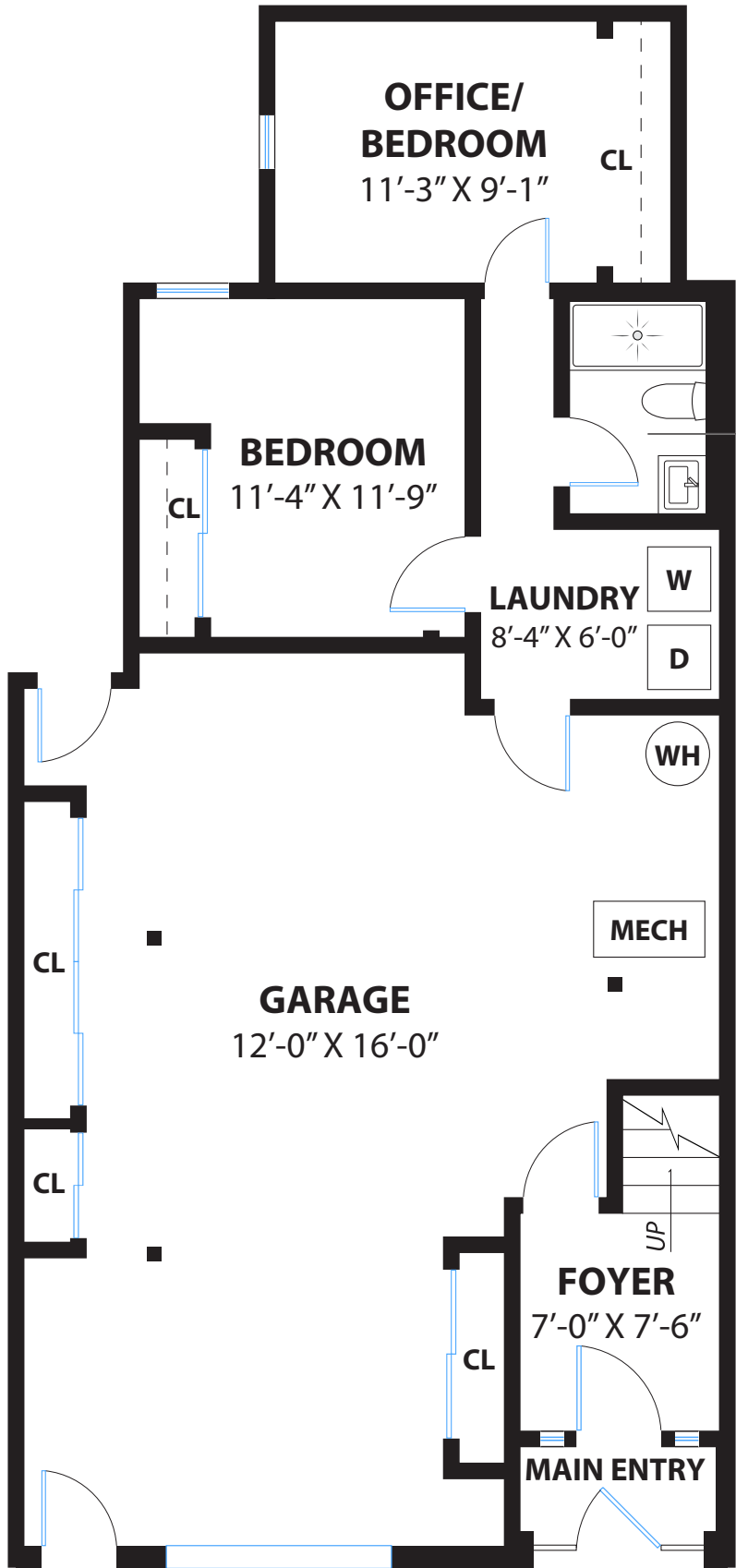
LOWER FLOOR
